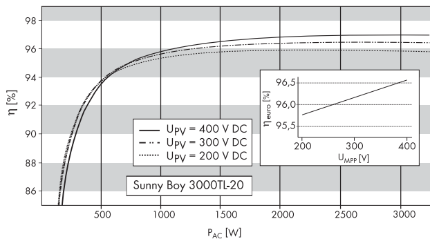
Efficiency curve
