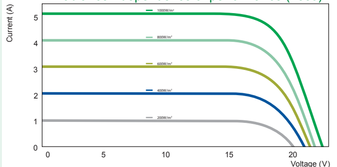
Irradiance - dependence of performance (485J)
